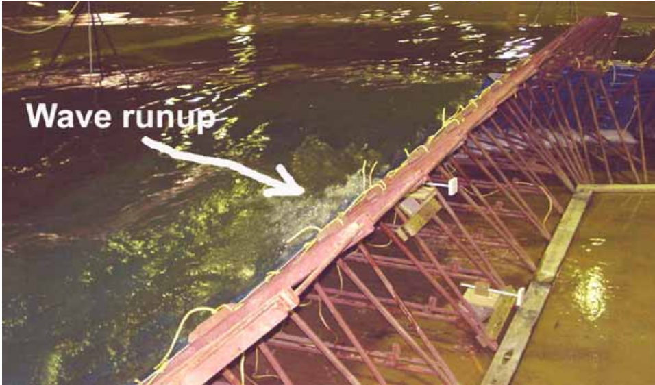
Figure 2-228. Wave action from high waves at 66 percent height, view inside left wall
