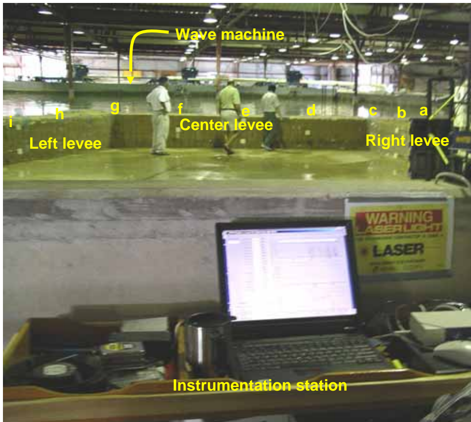
Figure 2-4. Laboratory setup
