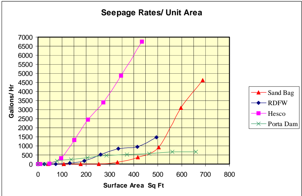
Figure 3-31. Seepage rate as a function of wetted perimeter area
