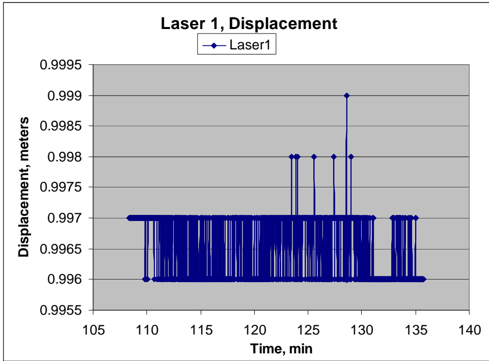
Figure 2-7c. Displacement data from laser 1
